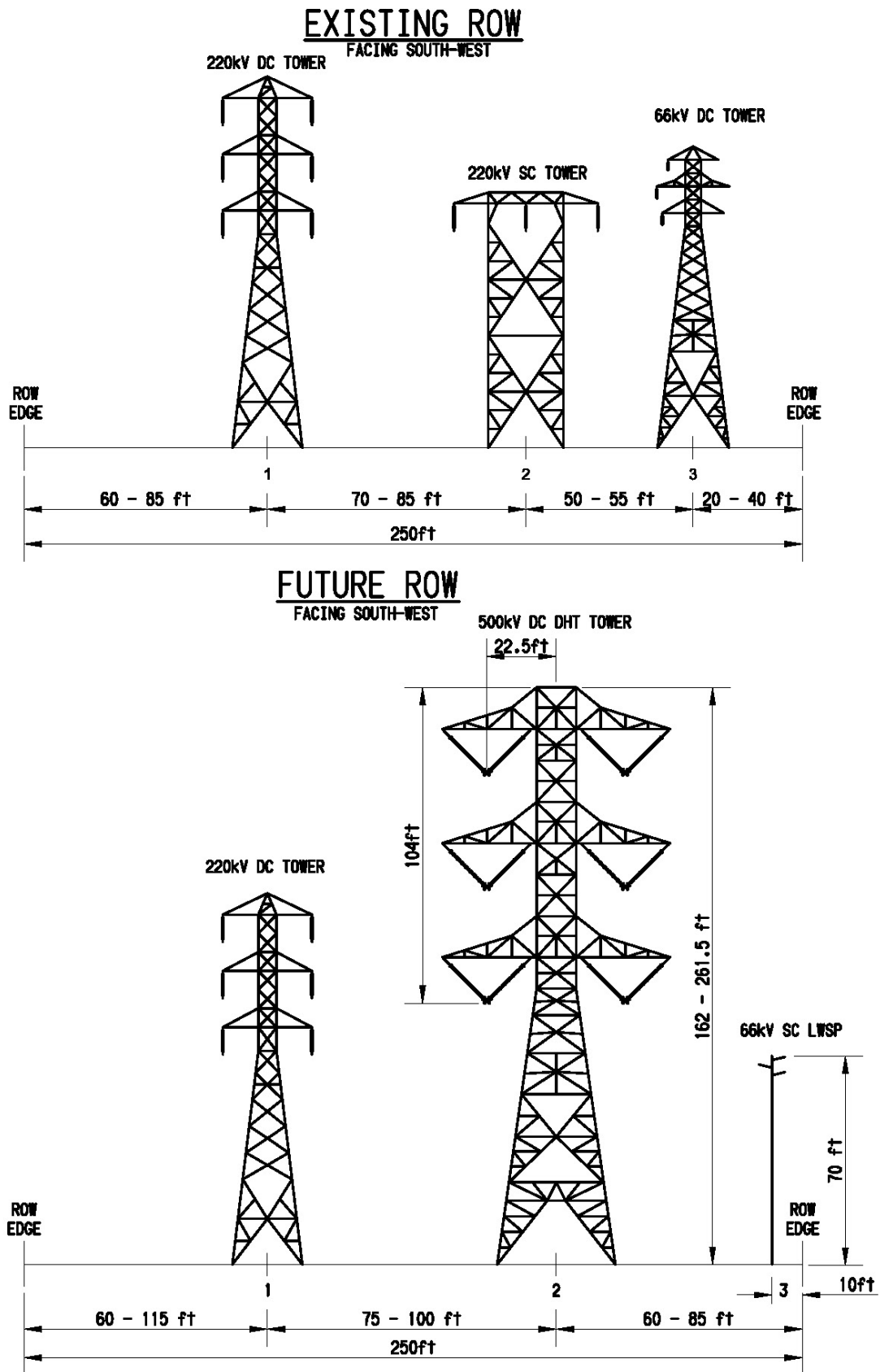
Figure 2.2-24 Segment 7 ROW Cross-Section (S7 MP 10.1 to S7 MP 10.5)
