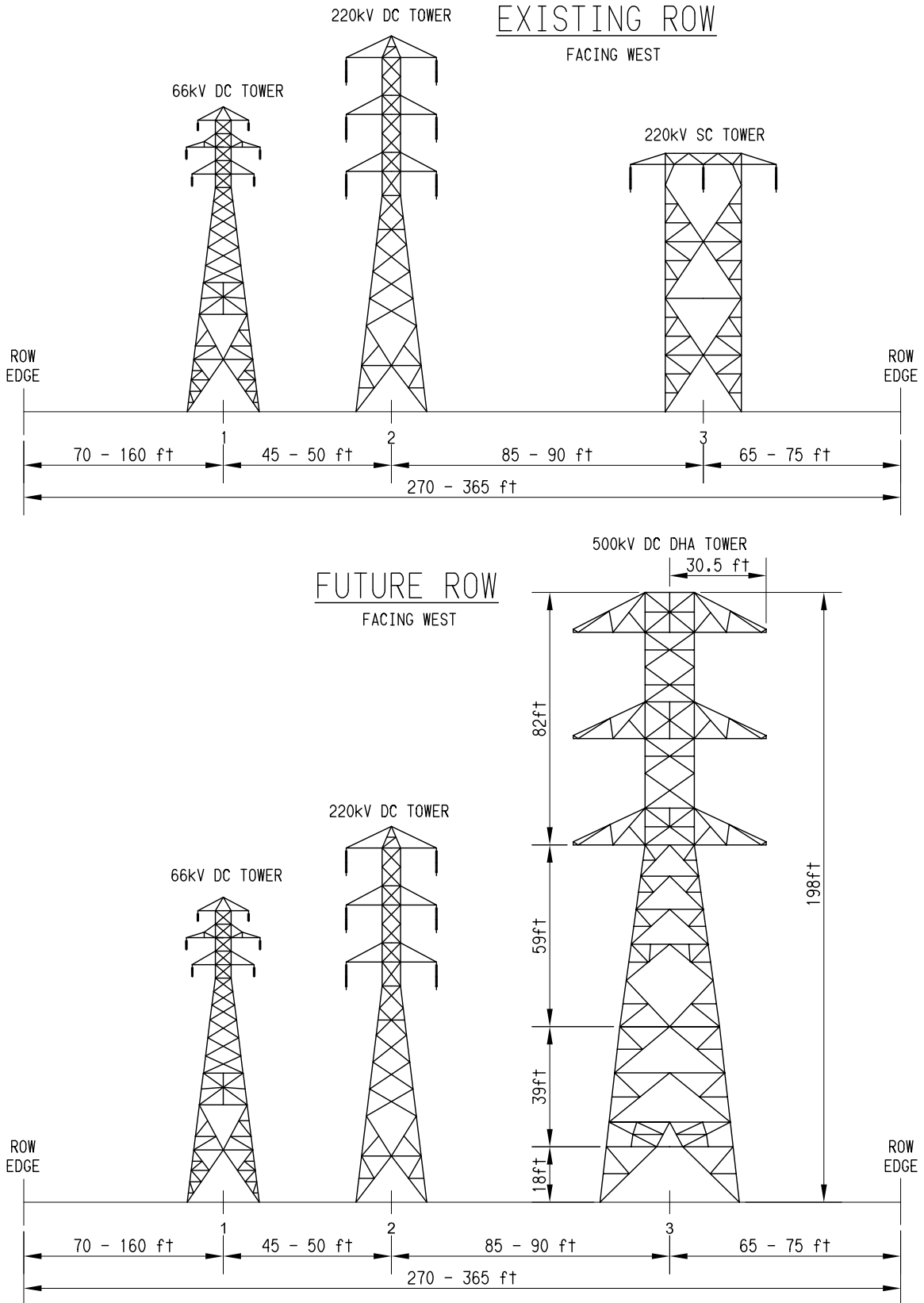
Figure 2.2-25 Segment 7 ROW Cross-Section (S7 MP 10.5 to S7 MP 10.95)
