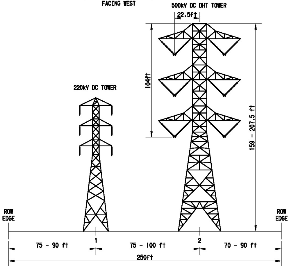
Figure 2.2-26a Segment 7 ROW Cross-Section (S7 MP 10.95 to S7 MP 11.8)
