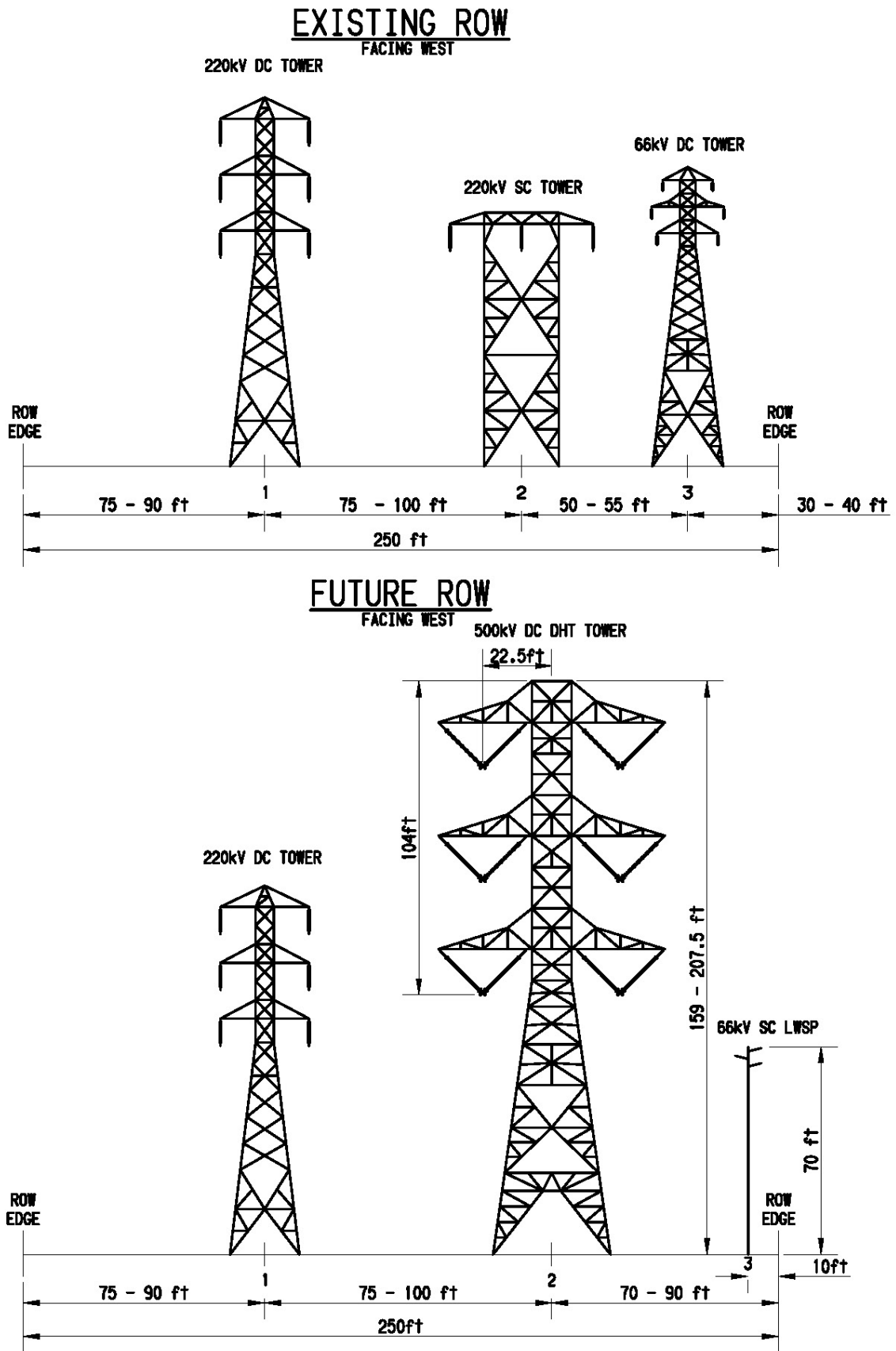
Figure 2.2-26b Segment 7 ROW Cross-Section (S7 MP 11.8 to S7 MP 13.4)
