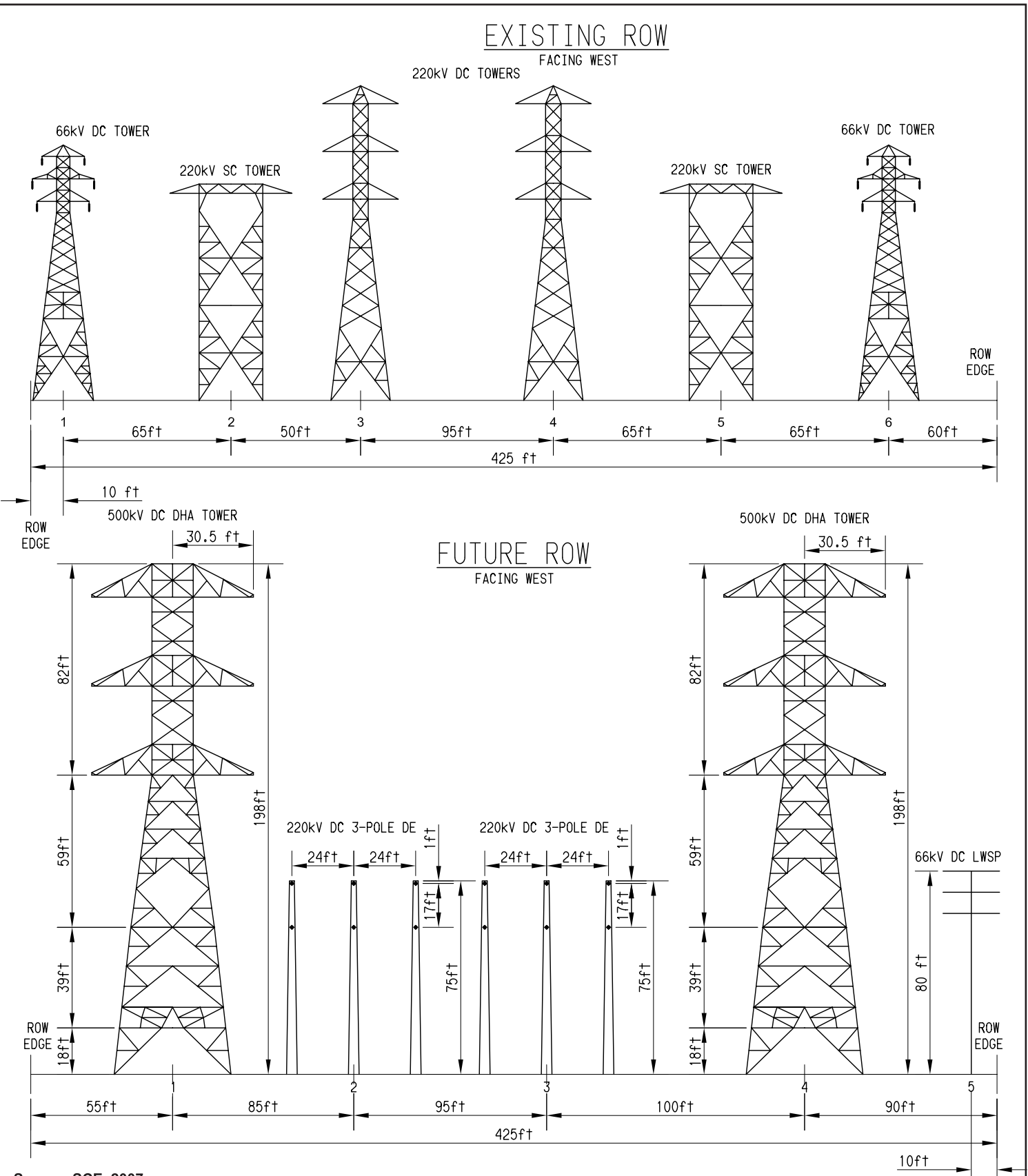
Figure 2.2-27 Segment 7 ROW Cross-Section (S7 MP 13.4 to S7 MP 13.7)
