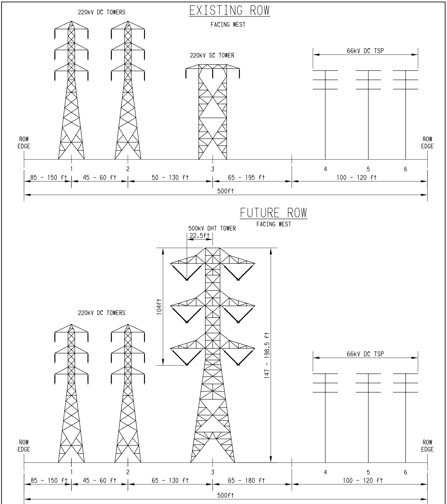
Figure 2.2-28 Segment 7 ROW Cross-Section (S7 MP 13.7 to S7 MP 15.8)
