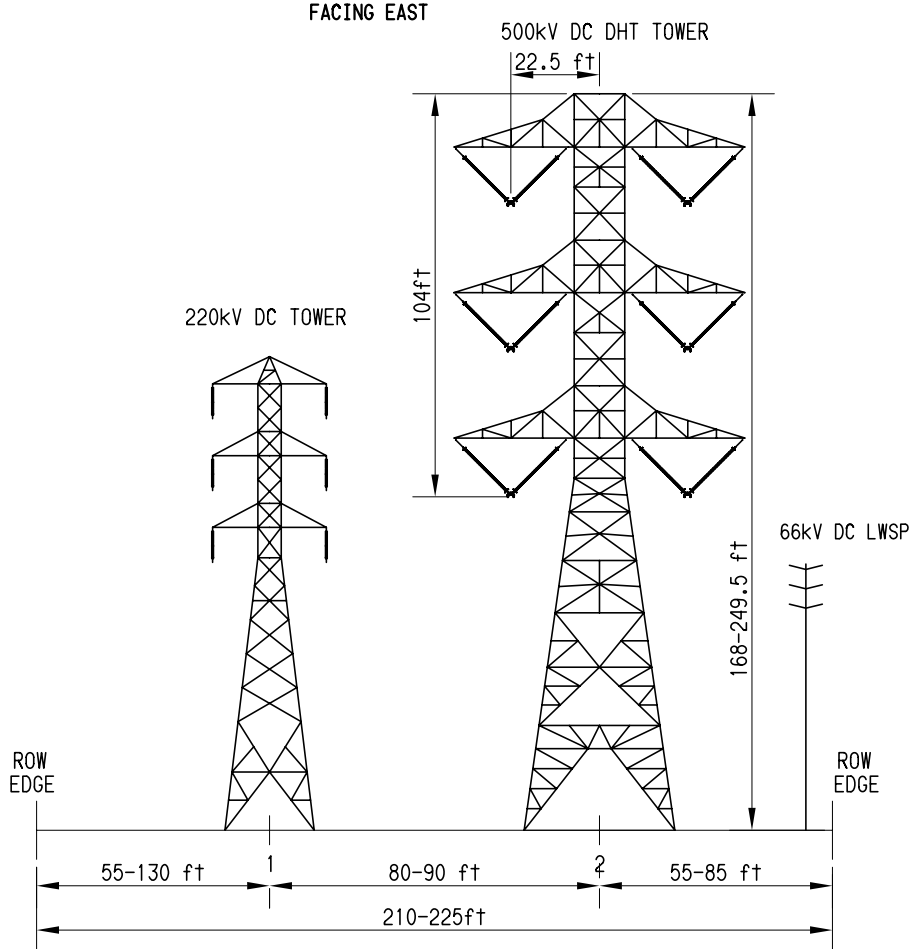
Figure 2.2-29 Segment 8 ROW Cross-Section (S8A MP 2.2 to S8A MP 4.2)
