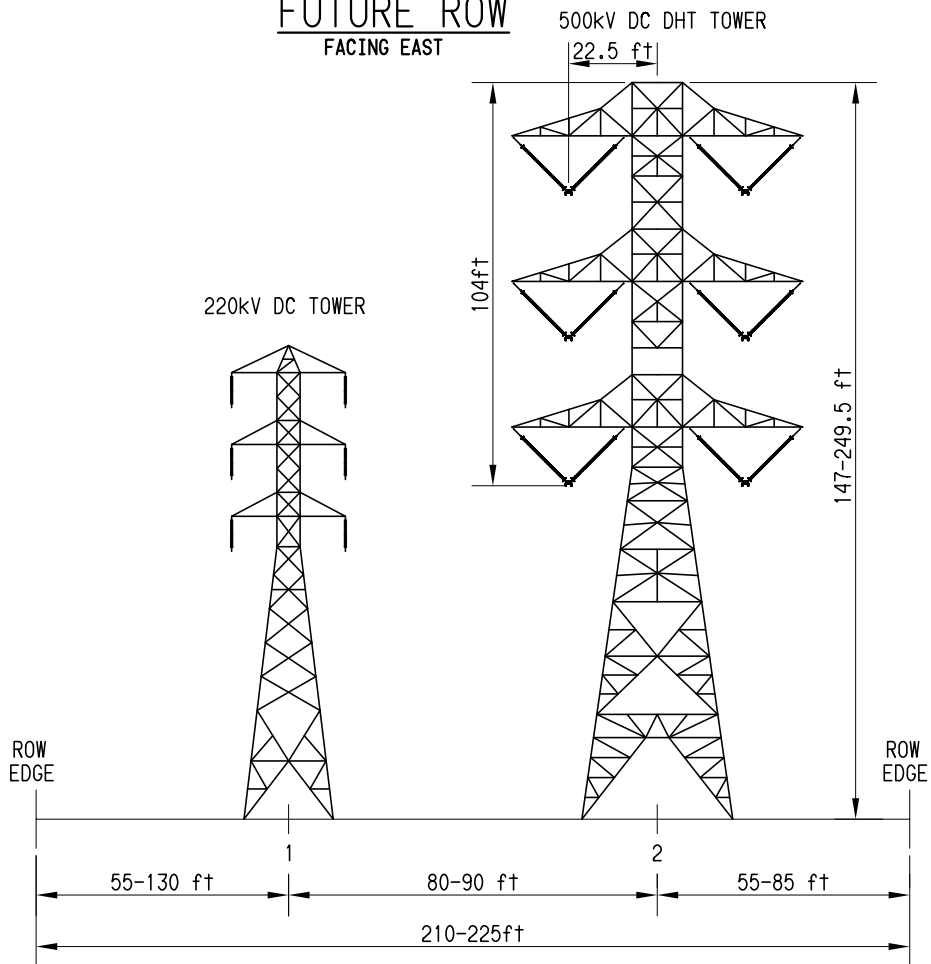
Figure 2.2-31 Segment 8 ROW Cross-Section (S8A MP 4.4 to S8A MP 5.85)
