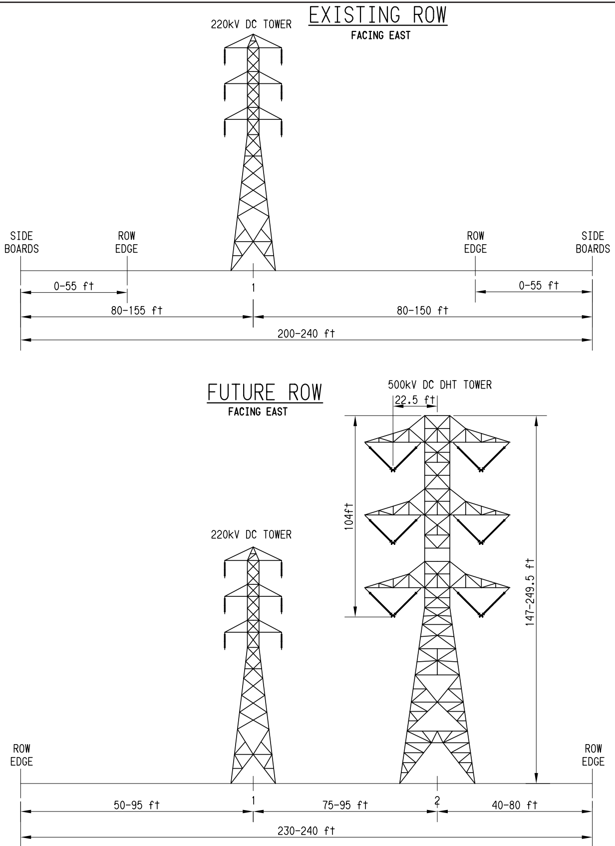
Figure 2.2-32 Segment 8 ROW Cross-Section (S8A MP 5.85 to S8A MP 8.1)
