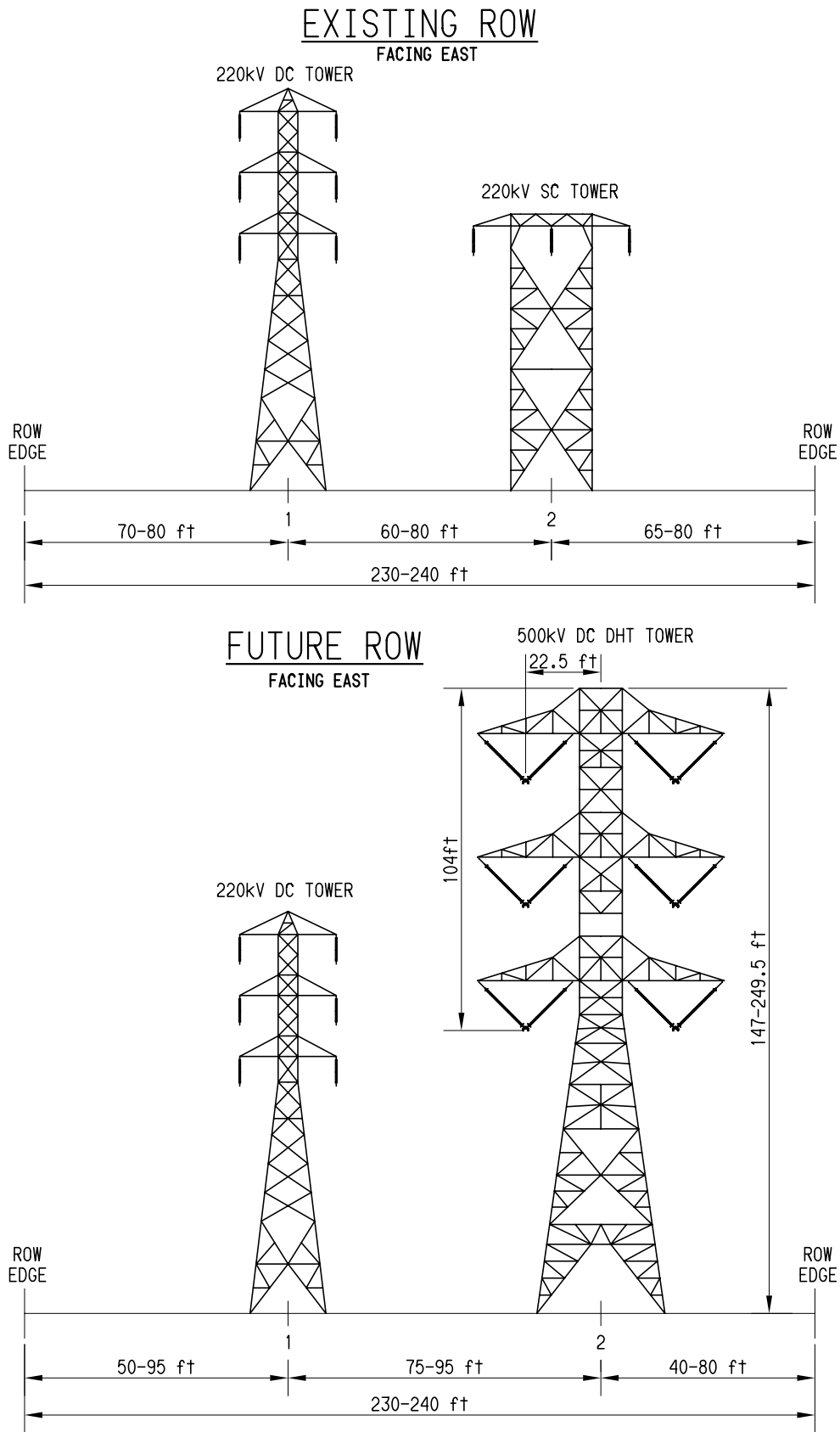
Figure 2.2-33 Segment 8 ROW Cross-Section (S8A MP 8.1 to S8A MP 9.0)
