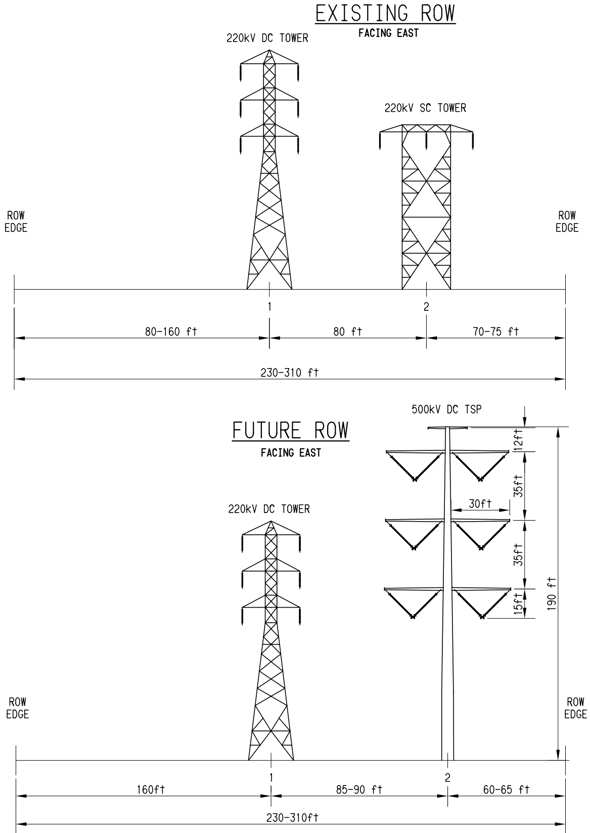
Figure 2.2-34 Segment 8 ROW Cross-Section (S8A MP 9.0 to S8A MP 9.5)
