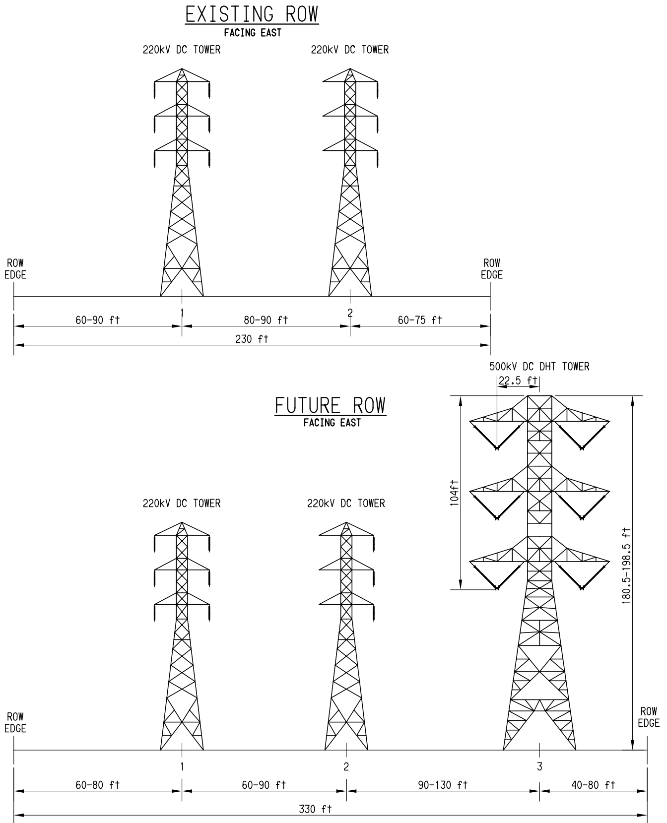
Figure 2.2-36 Segment 8 ROW Cross-Section (S8A MP 11.2 to S8A MP 13.3)
