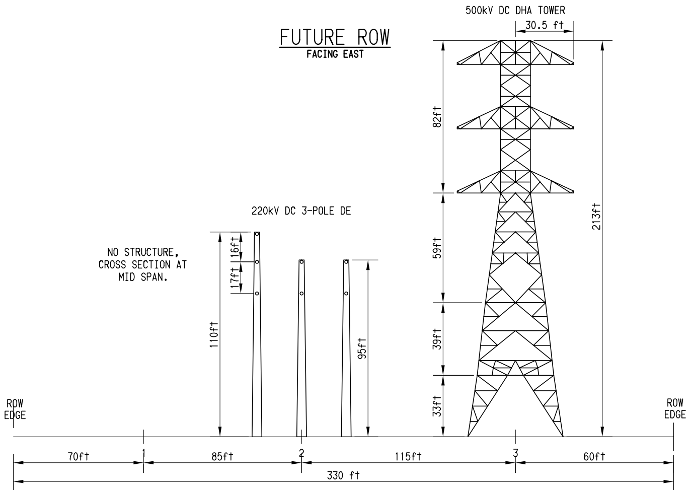
Figure 2.2-37 Segment 8 ROW Cross-Section (S8A MP 13.3 to S8A MP 13.4)
