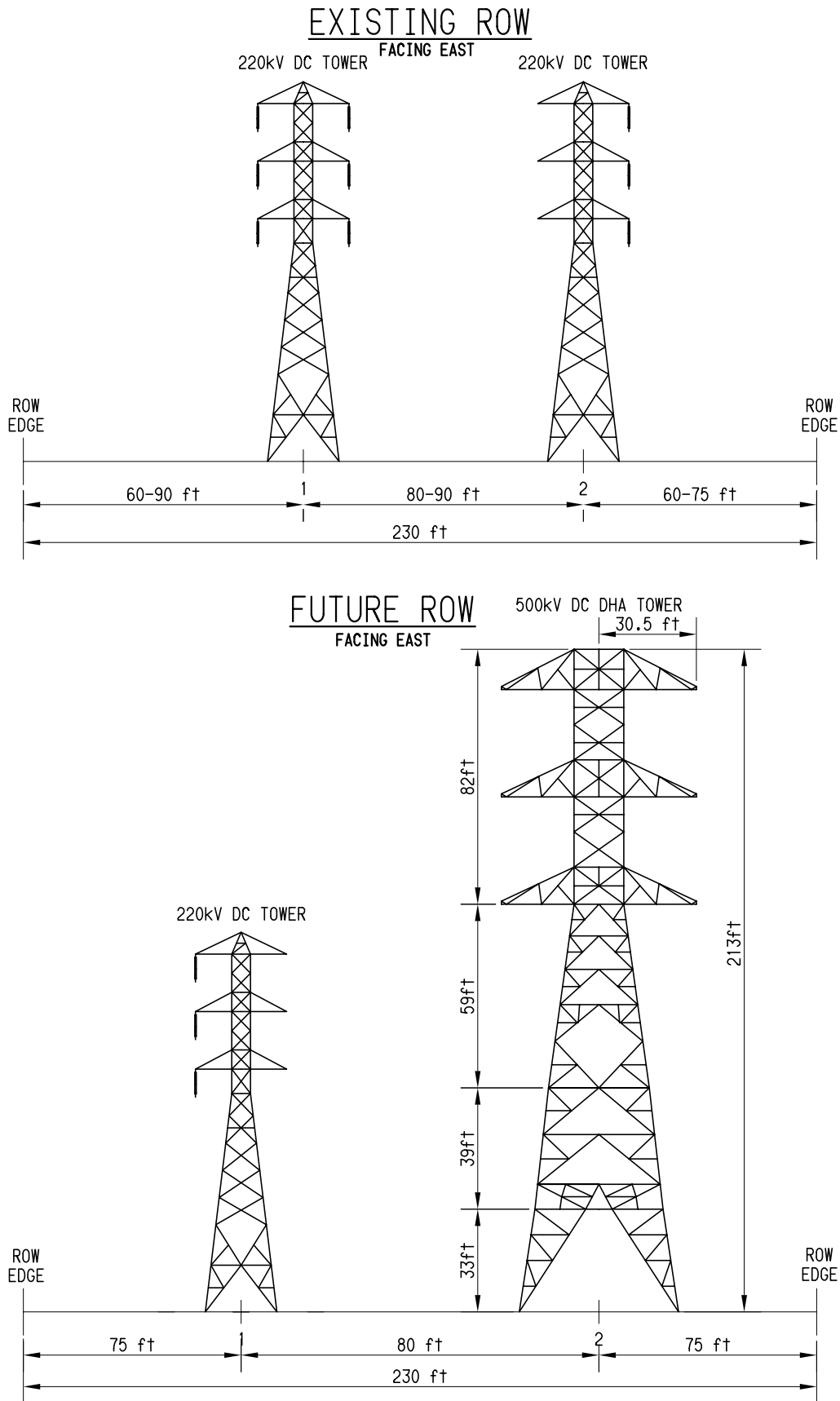
Figure 2.2-38 Segment 8 ROW Cross-Section (S8A MP 13.4 to S8A MP 13.55)
