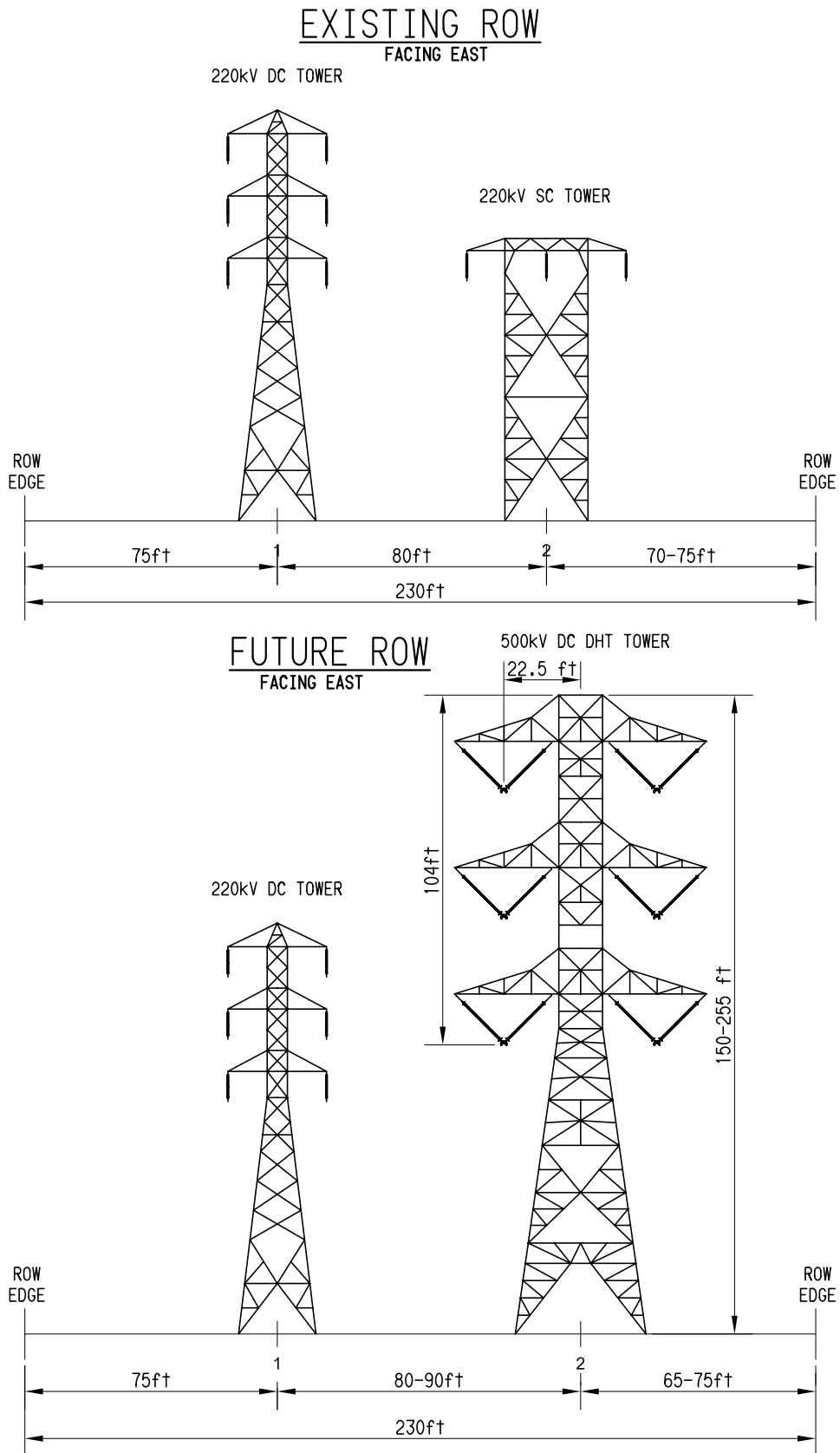
Figure 2.2-39 Segment 8 ROW Cross-Section (S8A MP 13.55 to S8A MP 19.2)
