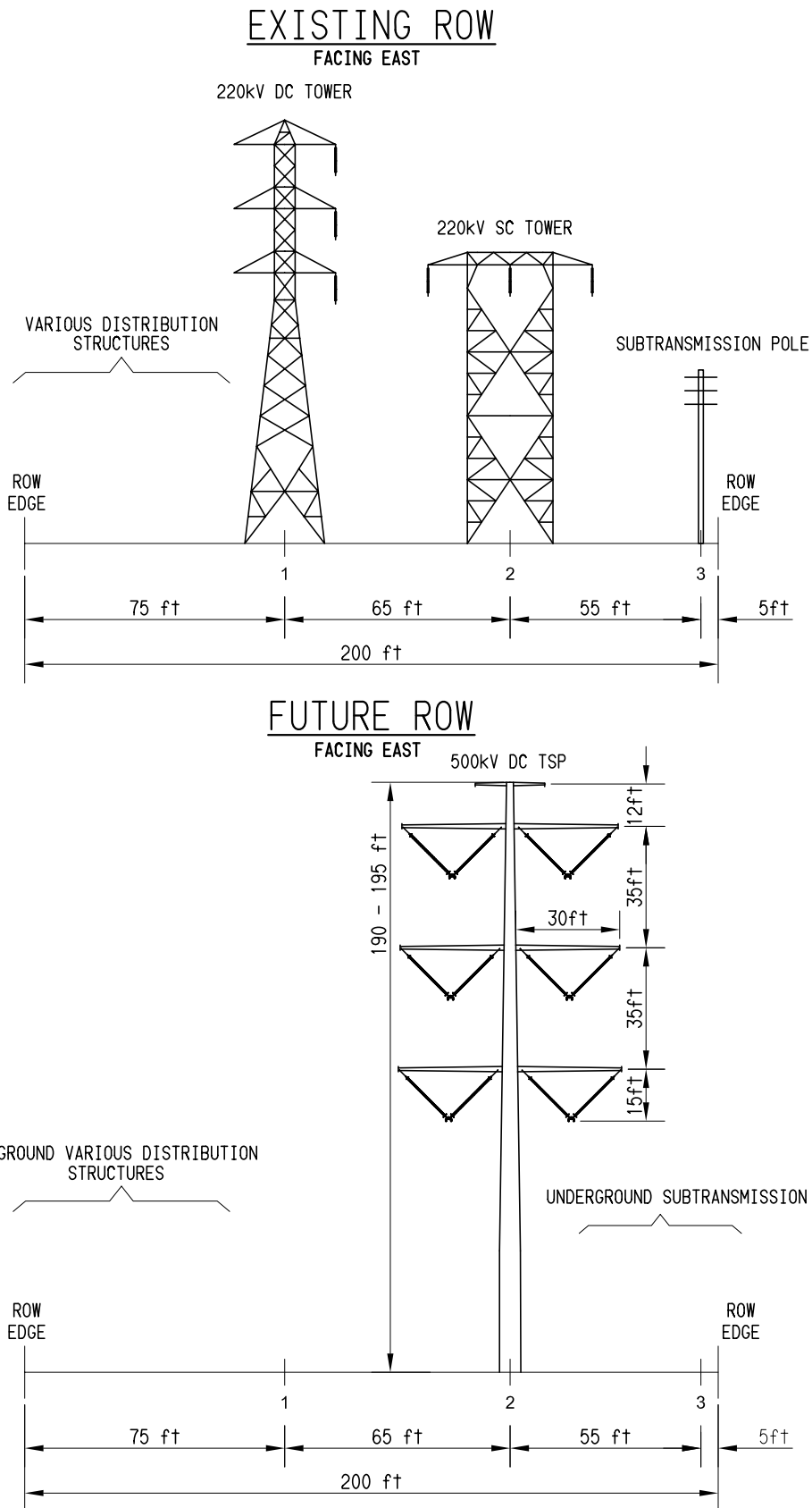
Figure 2.2-44 Segment 8 ROW Cross-Section (S8A MP 27.55 to S8A MP 28.3)
