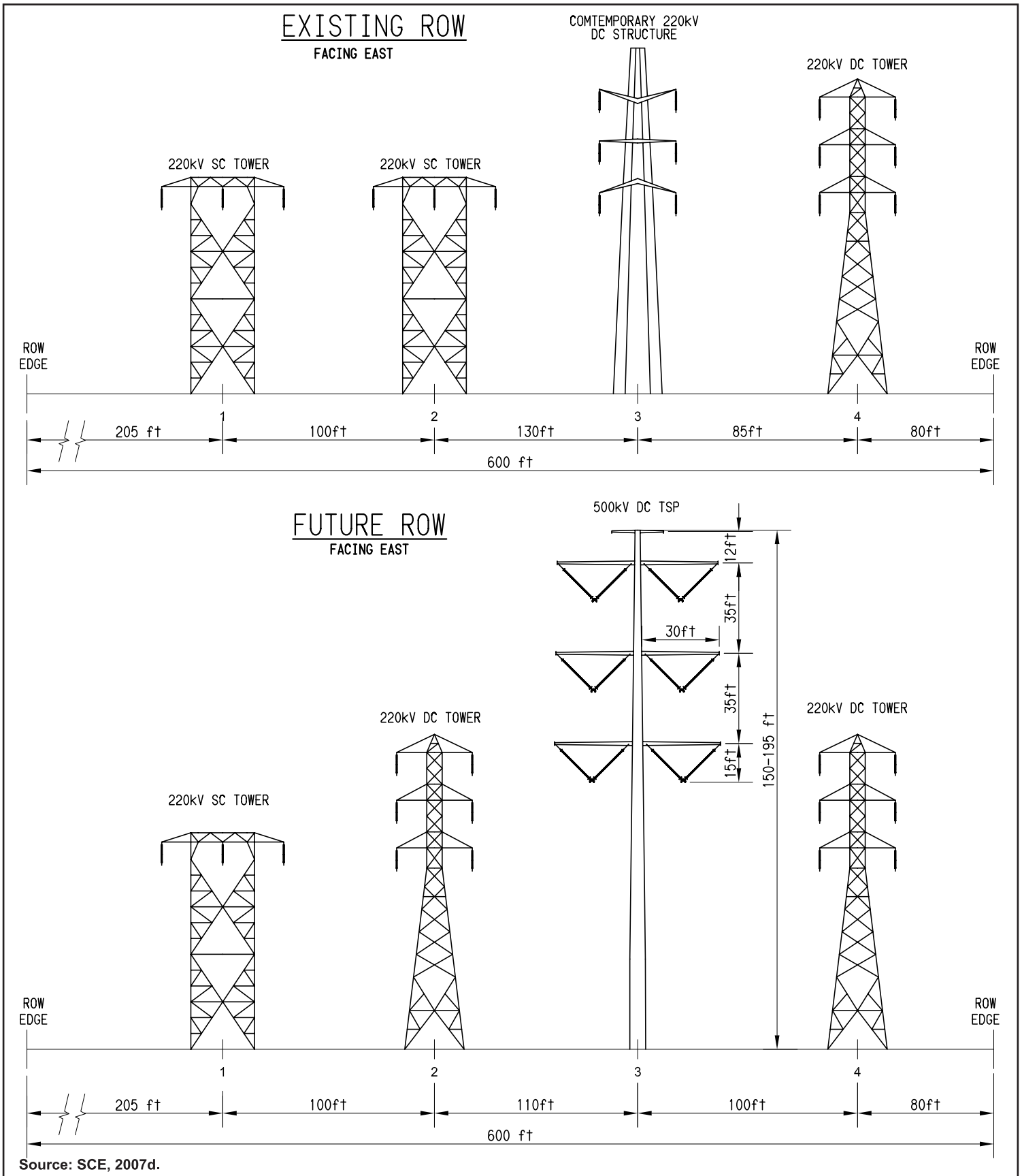
Figure 2.2-45 Segment 8 ROW Cross-Section (S8A MP 28.3 to S8A MP 29.2)
