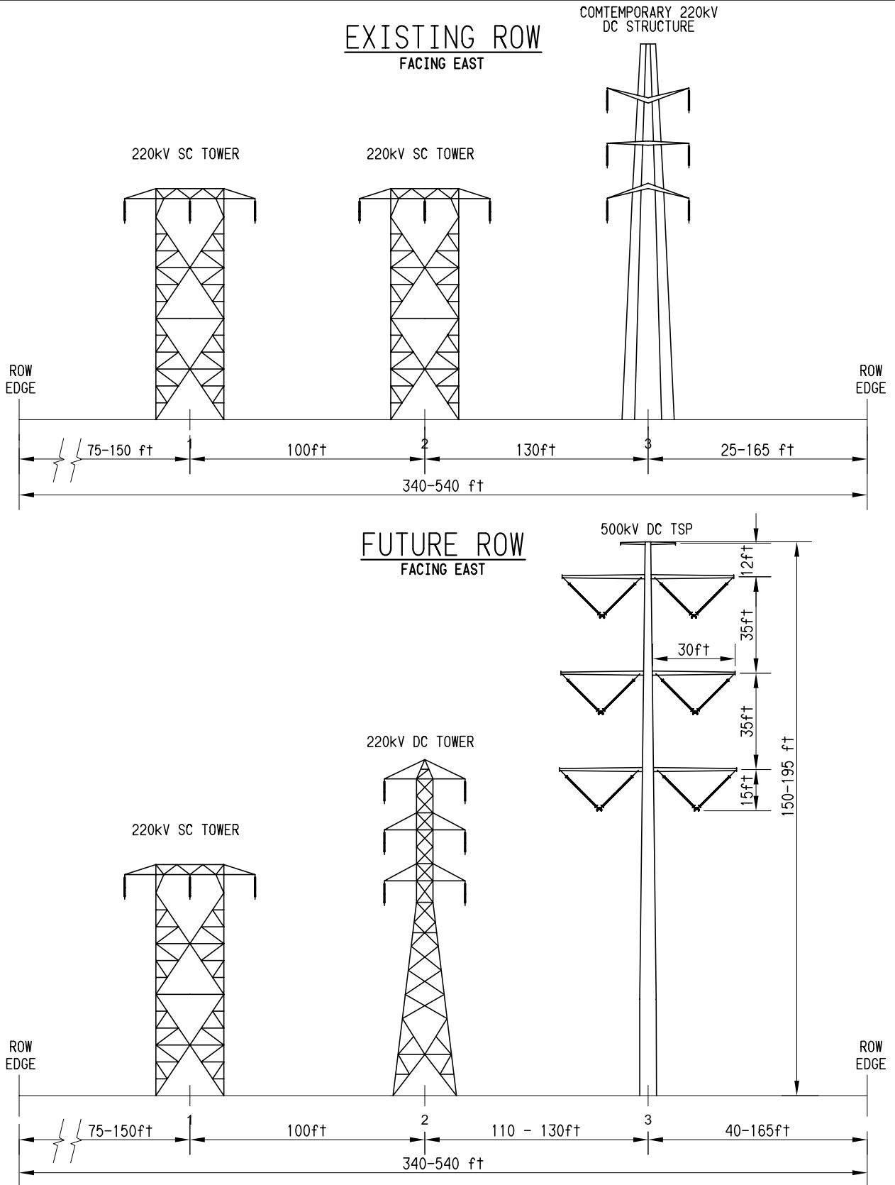
Figure 2.2-46 Segment 8 ROW Cross-Section (S8B MP 0.35 to S8B MP 0.75)
