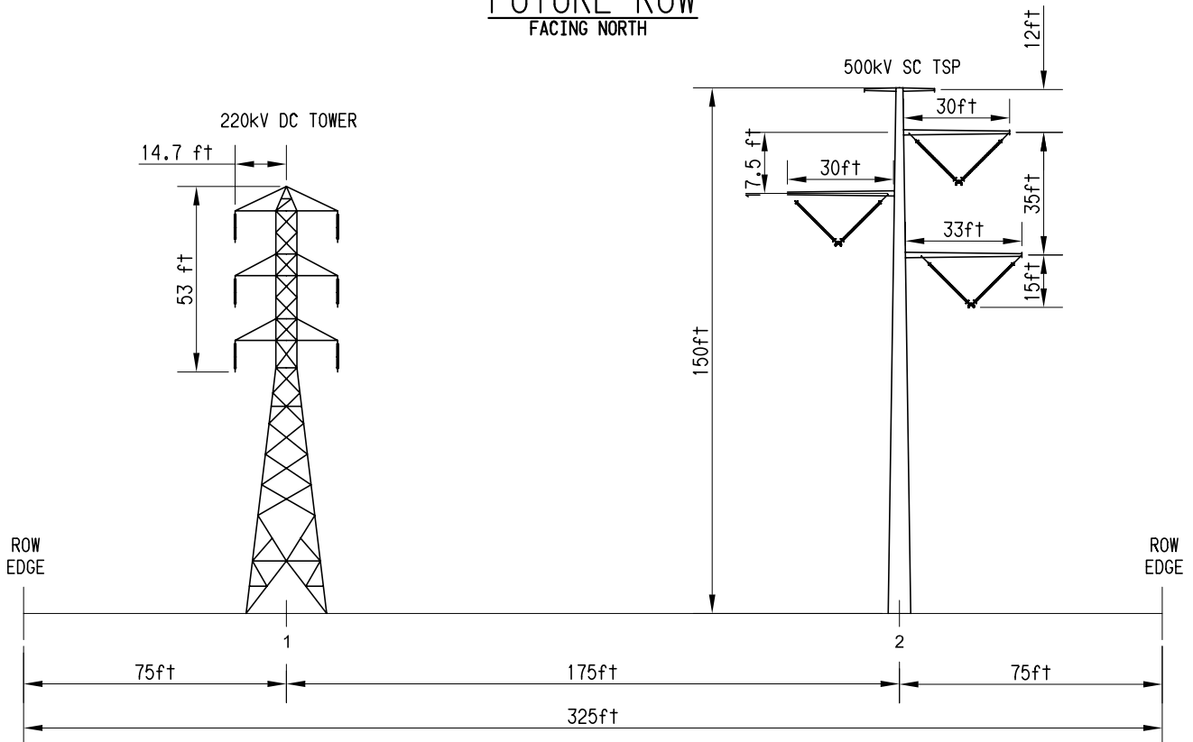
Figure 2.2-51 Segment 8 ROW Cross-Section (S8A MP 34.15 to S8A MP 34.4)
