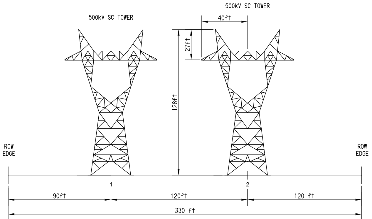
Figure 2.2-52 Segment 8 ROW Cross-Section (S8A MP 34.4 to S8A MP 34.5)
