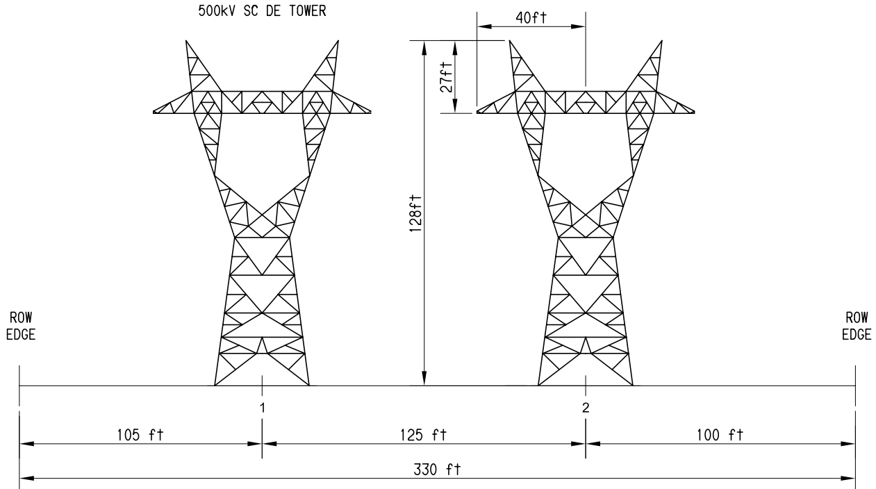
Figure 2.2-54 Segment 8 ROW Cross-Section (S8A MP 35.0 to S8A MP 35.2)
