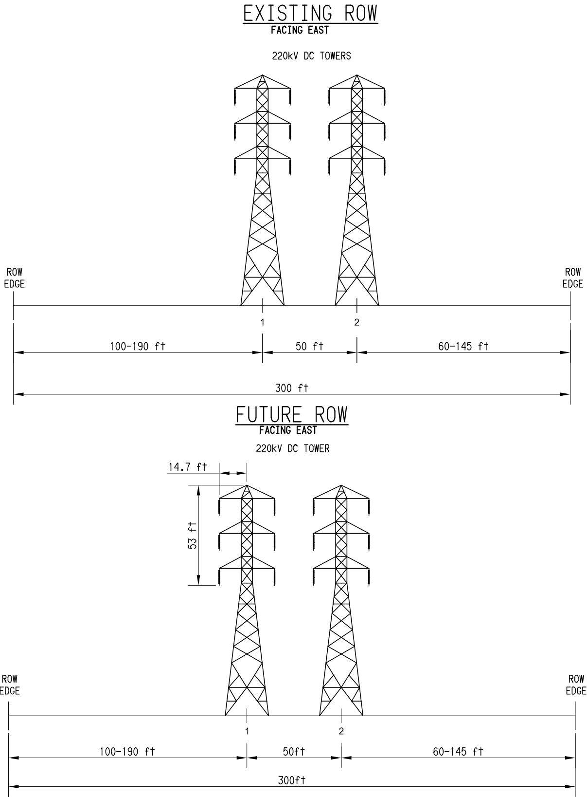
Figure 2.2-55 Segment 8 ROW Cross-Section (S8B MP 6.0 to S8B MP 6.8)
