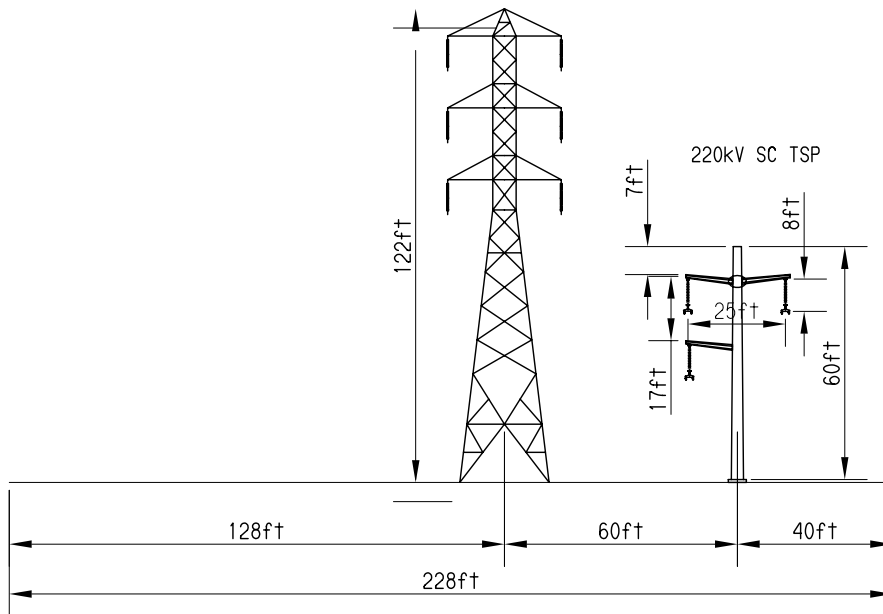
Figure 2.2-60 Segment 11 ROW Cross-Section (S11 MP 18.7 to S11 MP 18.85)
