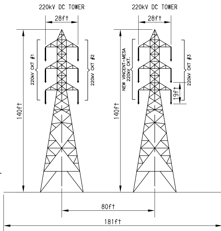
Figure 2.2-63 Segment 11 ROW Cross-Section (S11 MP 35.8 to S11 MP 36.2)
