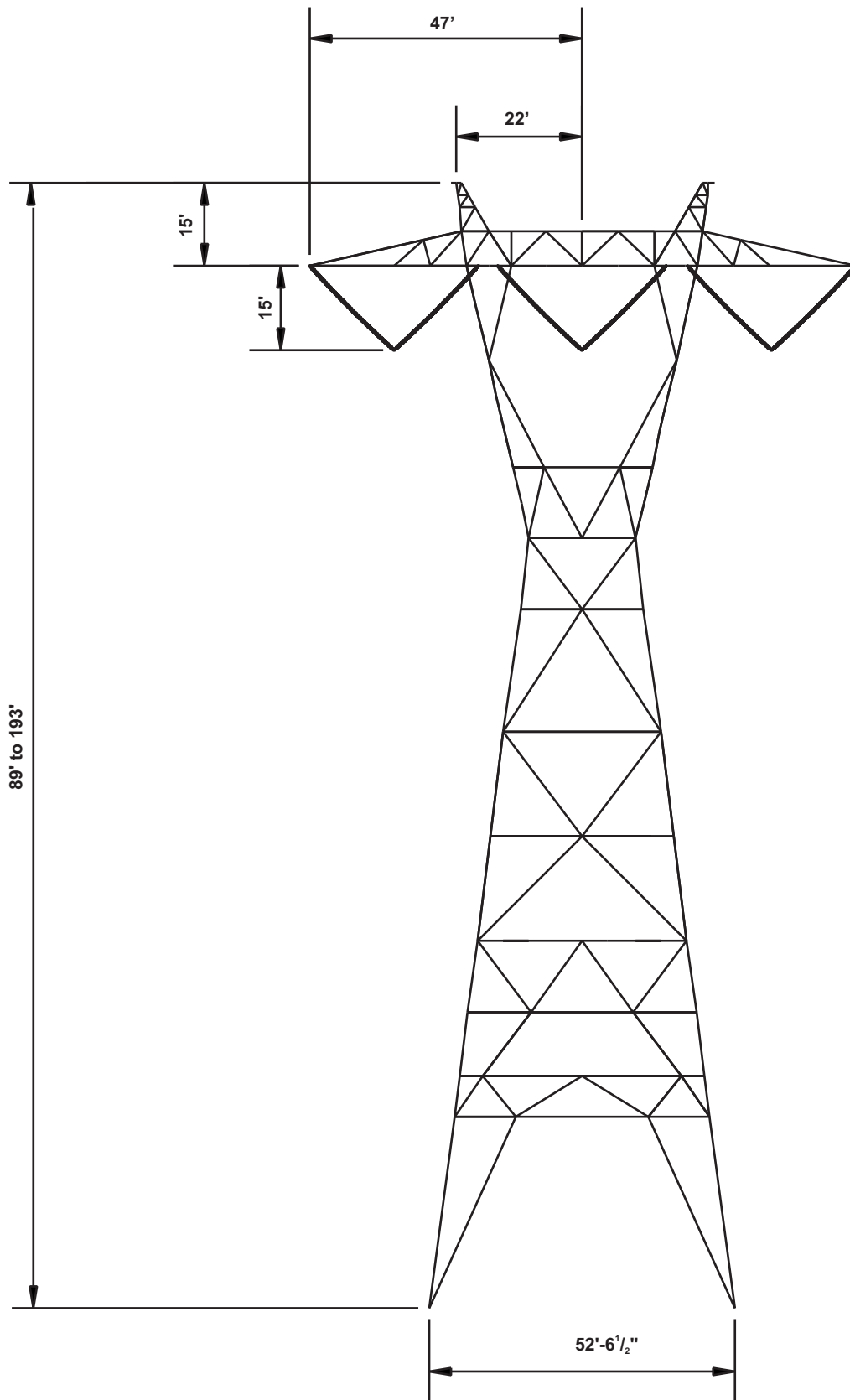
Figure 2.2-65 Typical 500-kV Single-Circuit Lattice Steel Tower
