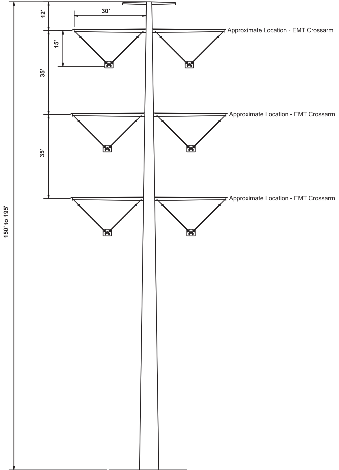
Figure 2.2-67 Typical 500-kV Double-Circuit Tubular Steel Pole
