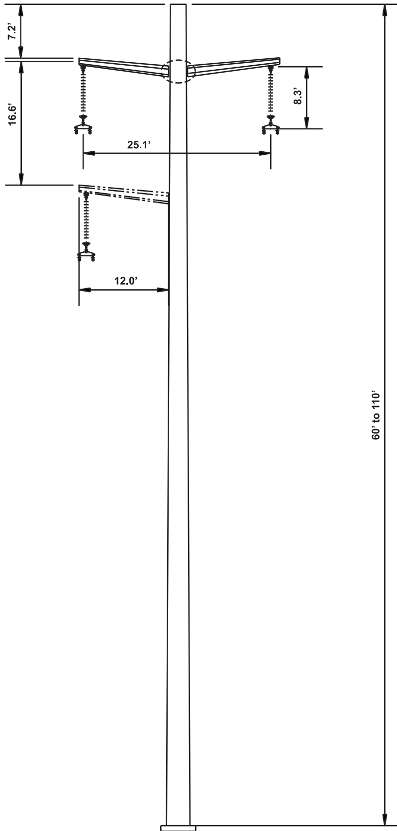
Figure 2.2-74 Typical 220-kV Single-Circuit Tubular Steel Pole
