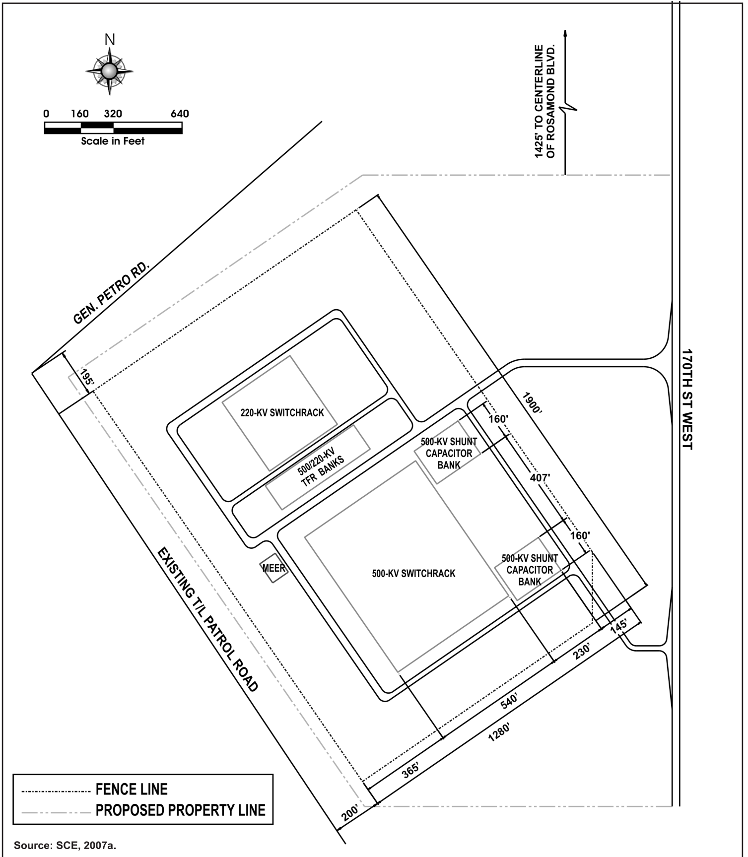
Figure 2.2-75 Proposed New Whirlwind Substation
