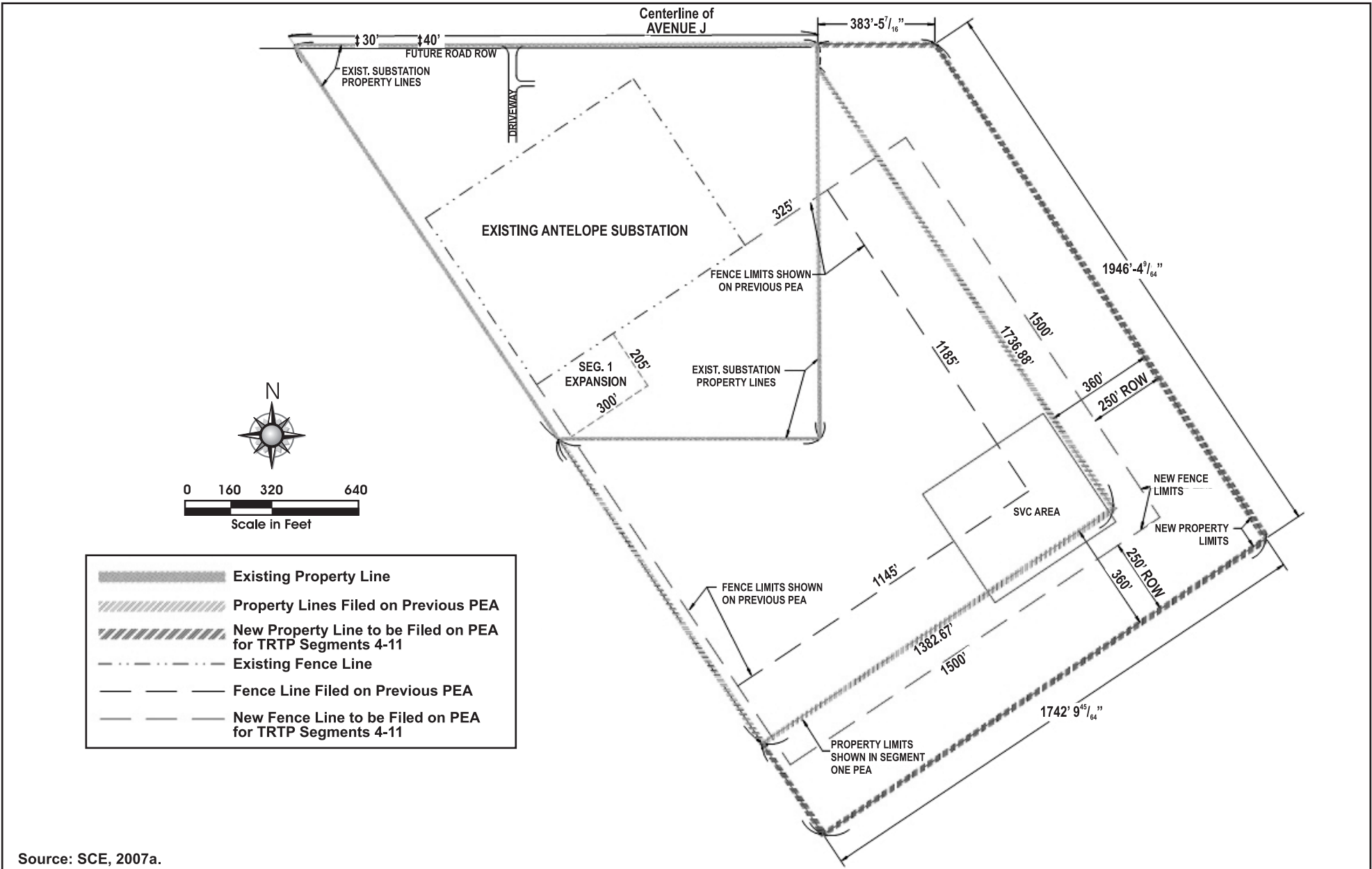
Figure 2.2-76 Proposed Upgrades to Antelope Substation
