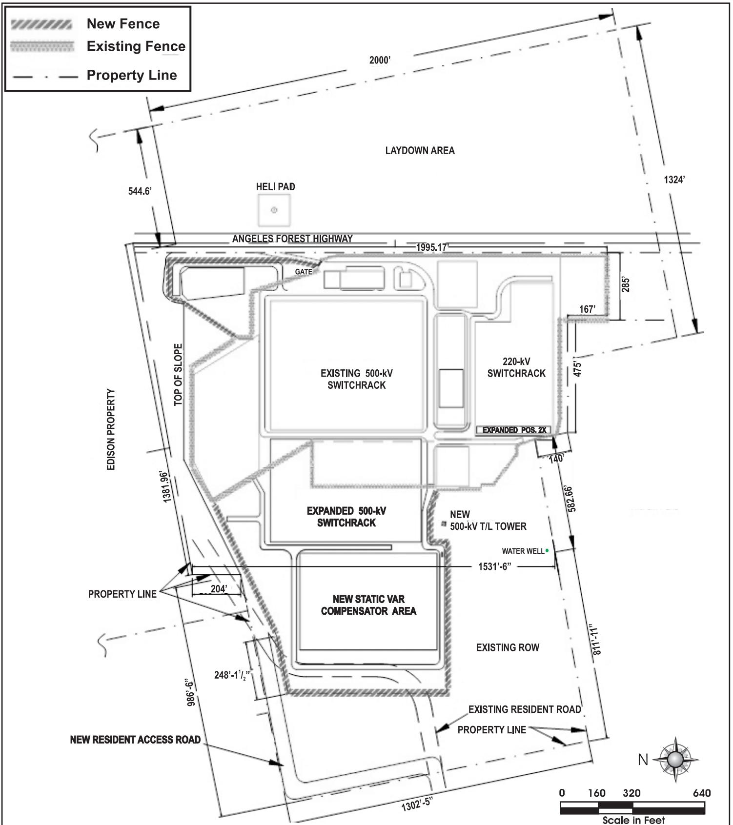
Figure 2.2-77 Proposed Upgrades to Vincent Substation
