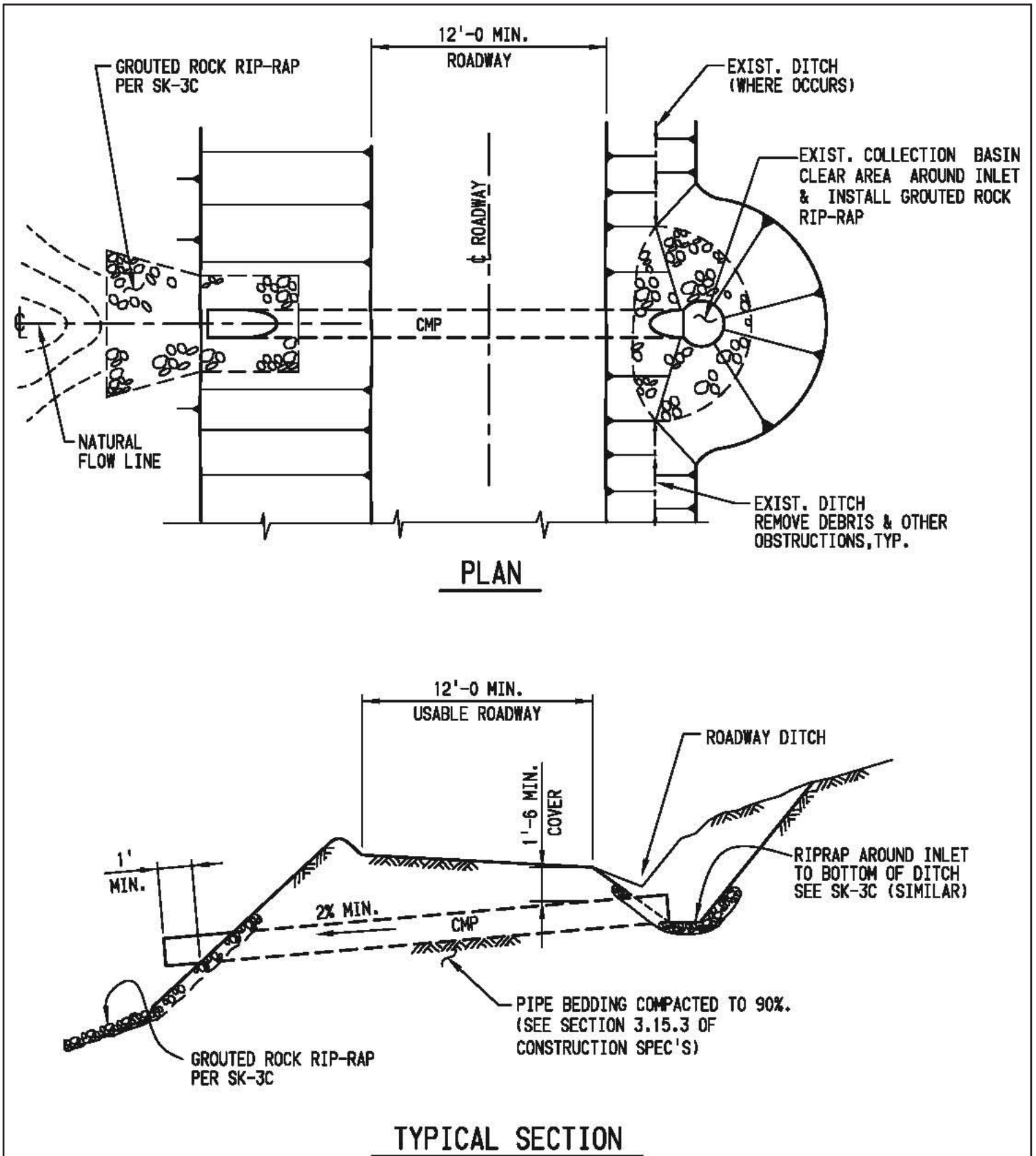
Figure 2.2-81 Pipe Culvert Installation
