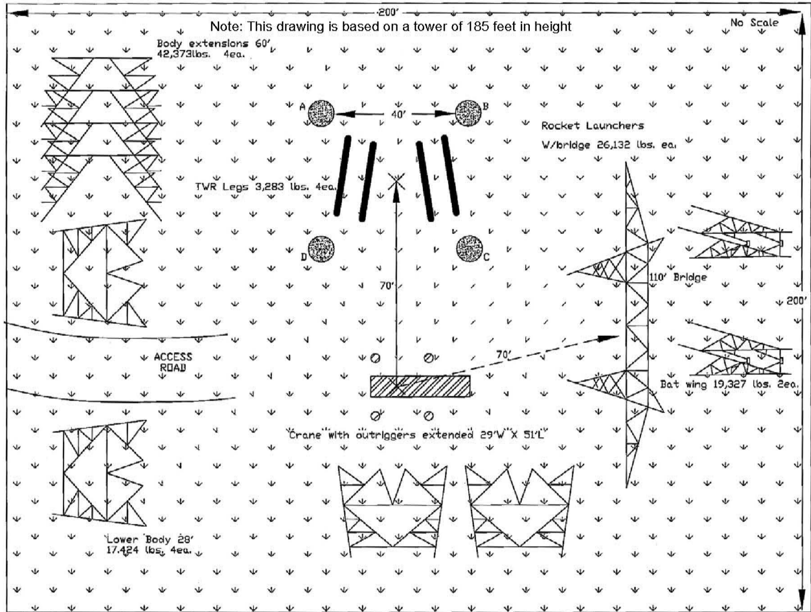
Figure 2.2-85 Typical Lattice Steel Tower Assembly Area
