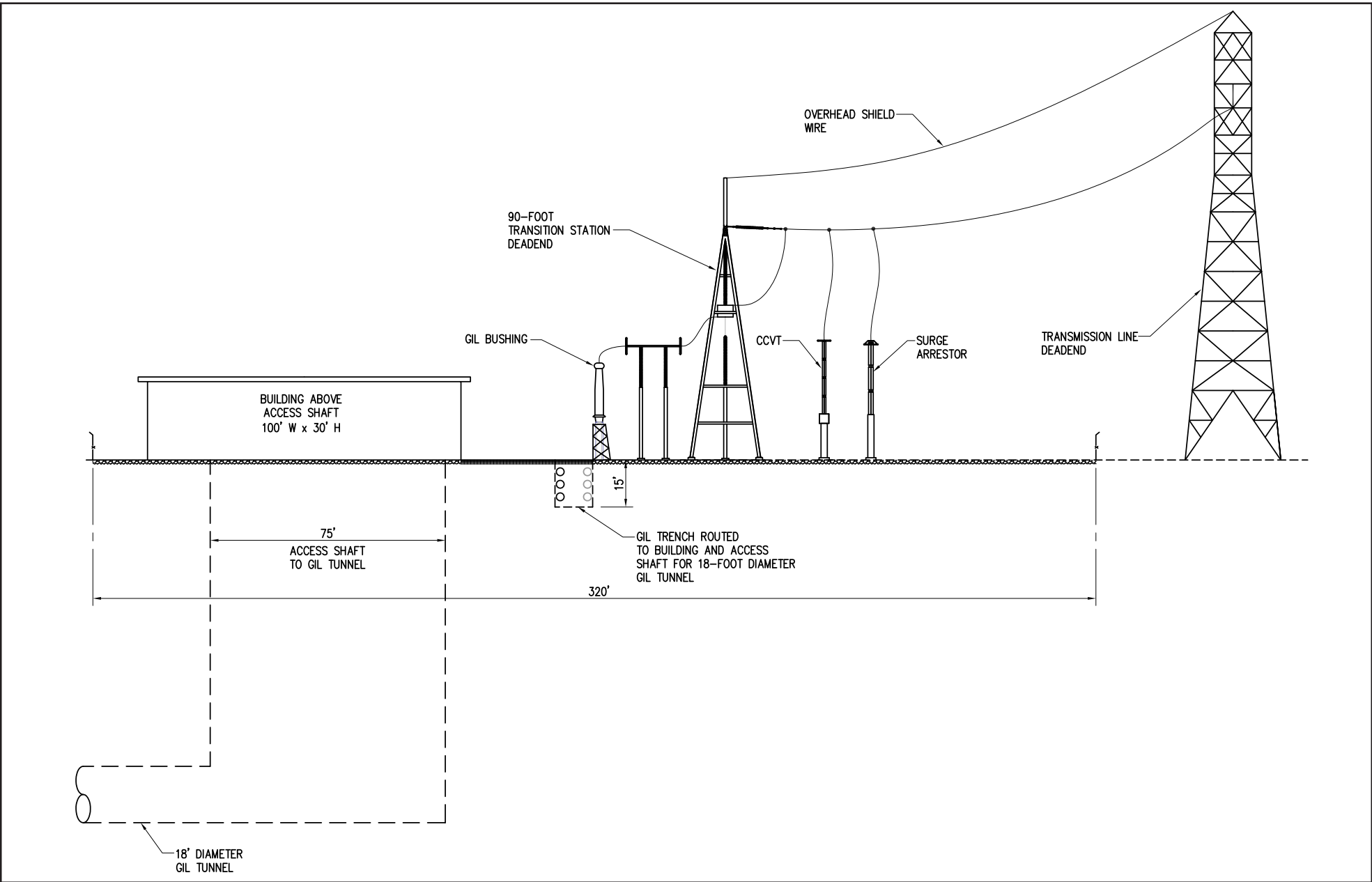
Figure 2.5-4 GIL Transition Station Side Elevation
