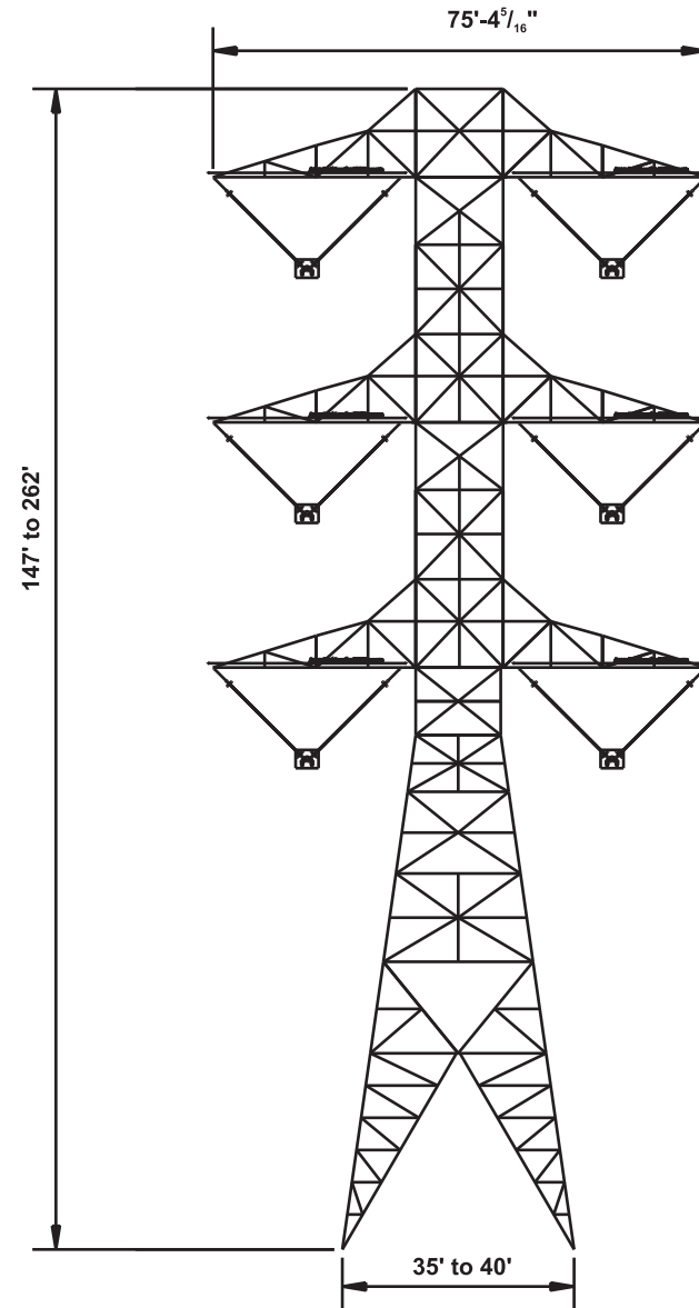
Figure 11 Typical 500-kV Lattice Steel Towers
