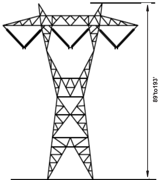
500-kV Single-Circuit Lattice Steel Tower
