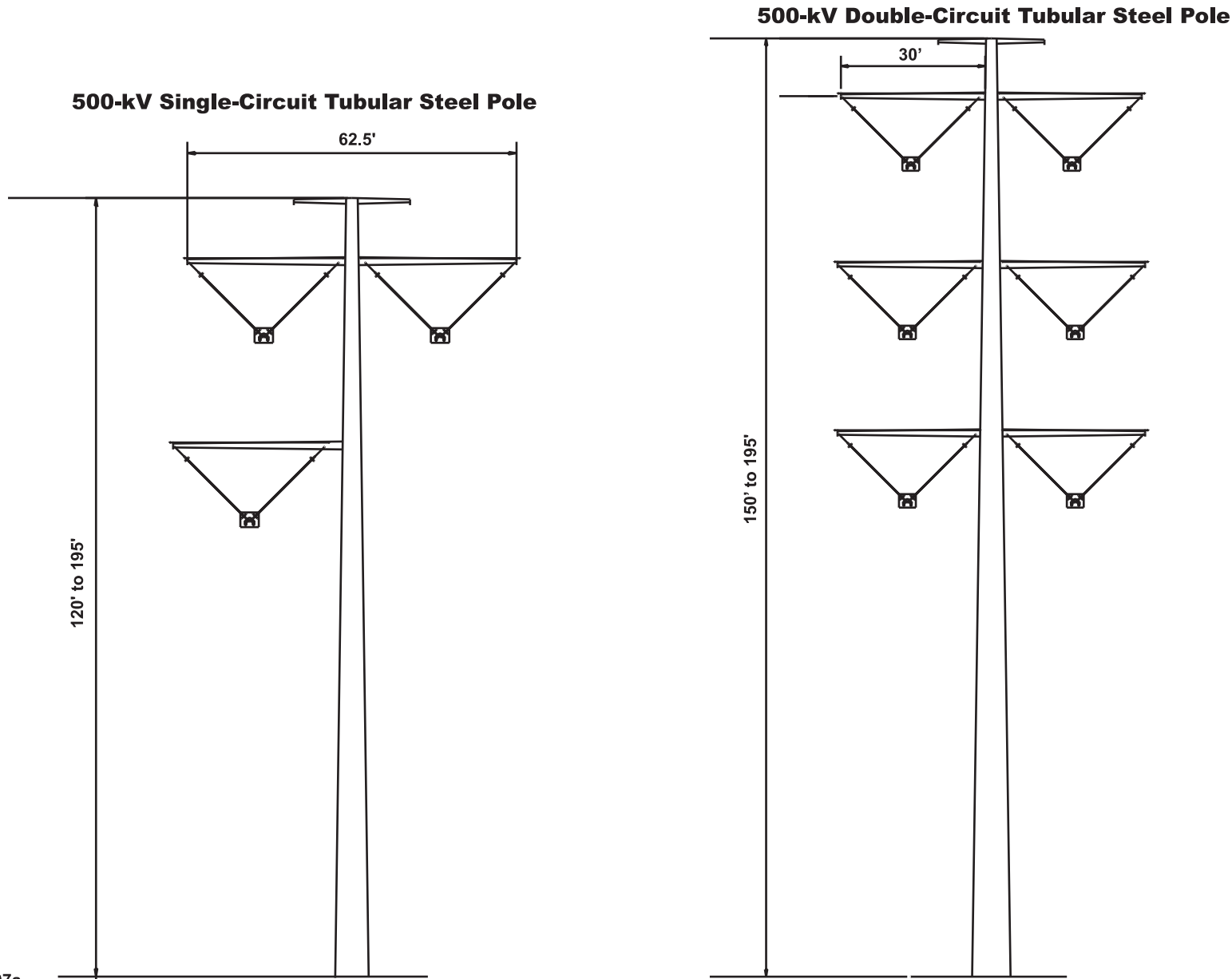
Figure 12 Typical 500-kV Tubular Steel Poles
