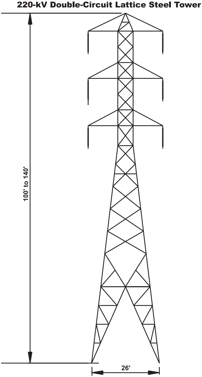
Figure 13 Typical 220-kV Lattice Steel Towers
