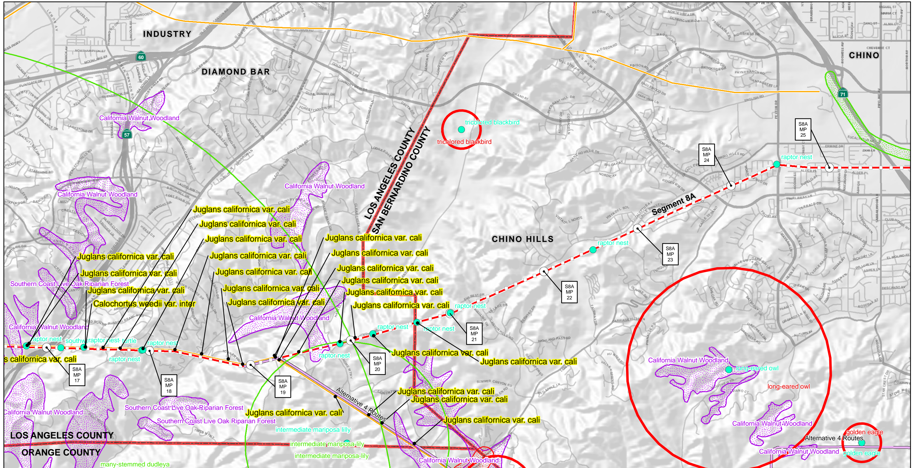
Figure 3.4-5x Sensitive Species Locations Southern Region
