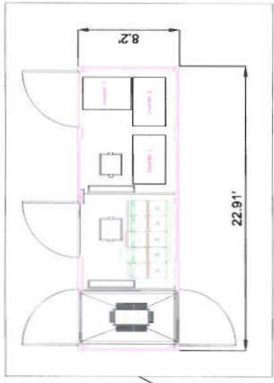
TRANSFORMER + INVERTERS
